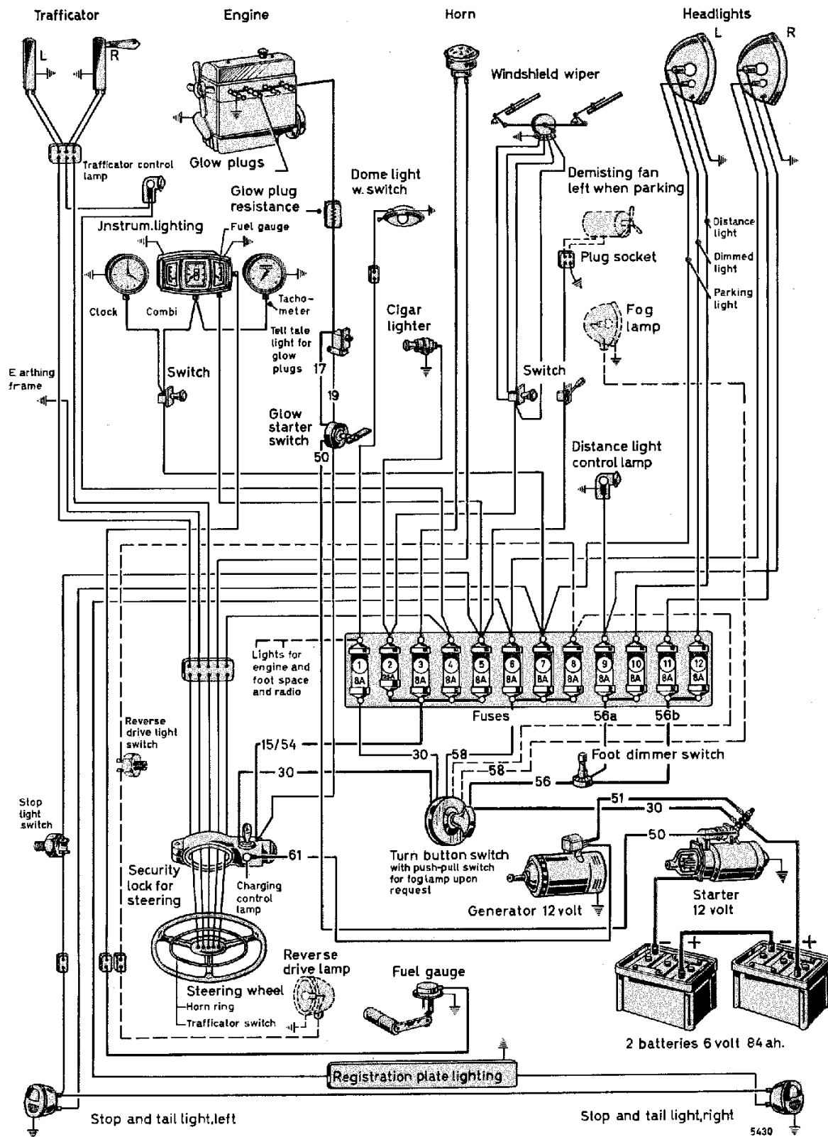
Wiring diagram for the electrical fittings
