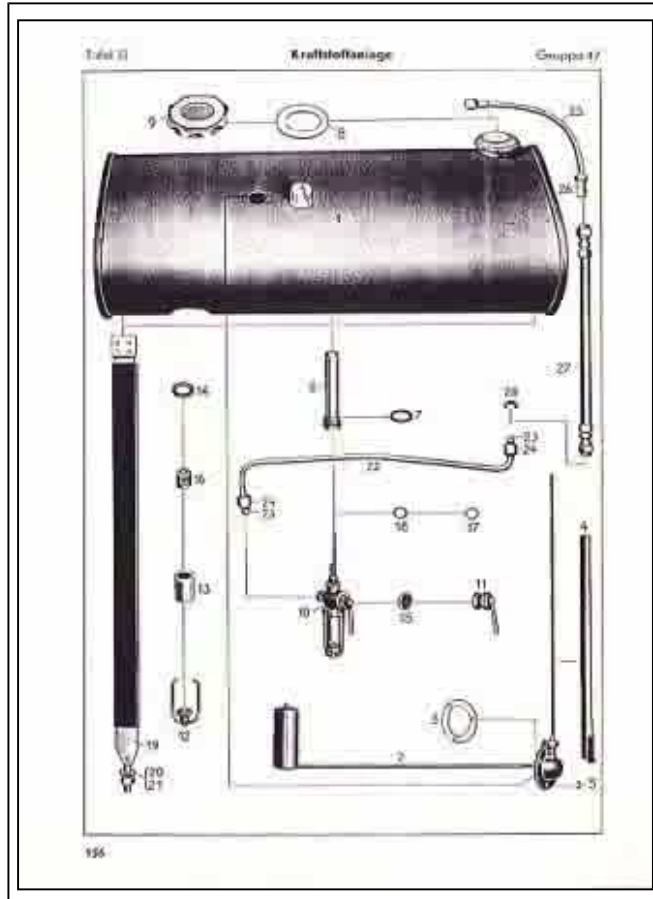
170V Fuel Tank Diagram
